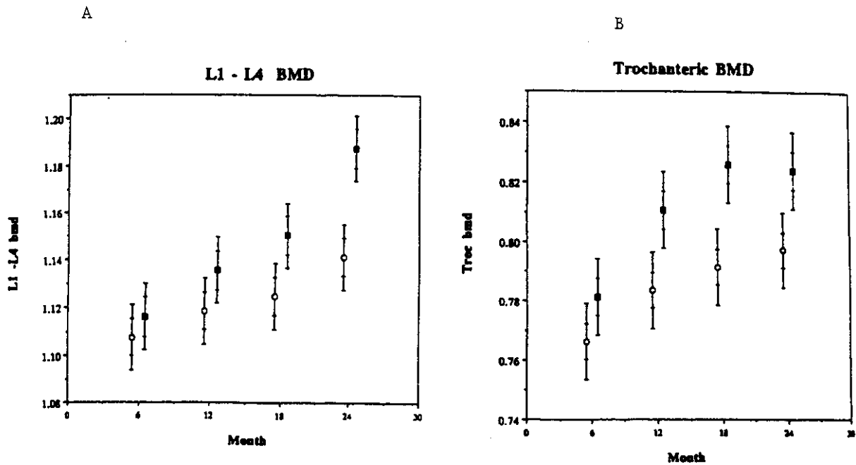
Fig. 8. The effect of hormonal implants on bone mineral density (gm/cm 2 ) in (A) the lumbar spine (L1-L4) and (B) the femoral trochanter (Troc); estradiol = E, (○); estradiol plus testosterone = E + Te (■). Error bars represent standard error of the differences between means (SED). Inner error bars are used to compare means between times for the same treatment. The comparison between the treatment groups is made with the outer error bars. If error bars do not overlap, i.e., differ by more than 2 SED, the means are significantly different by a P value of at least .05. Adapted from Davis SR, McCloud PI, Strauss BJJ et al. Testosterone enhances estradiol's effects on postmenopausal bone density and sexuality. Maturitas 1995;21:227-236, © 1995, used with permission from Elsevier Science (42).
