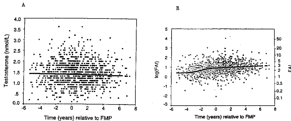
Fig. 5. A, linear regression model: observed testosterone ( T ) and fitted levels of mean T across the menopausal transition. B, double logistic model: observed FAI and fitted levels of mean FAI across the menopausal transition. The left and right axes show FAI levels on the log and antilog scales, respectively. The horizontal axis represents time (years) with respect to FMP ( \circ ); negative (positive) numbers indicate time before (after) FMP. Adapted from (17) used with permission © The Endocrine Society.
