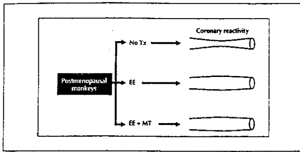
Fig. 14. Effect on acetylcholine-induced coronary artery dilation of adding methyltestosterone to esterified estrogens. Tx, treatment; EE, esterified estrogens; MT, methyltestosterone. Adapted from (78).
